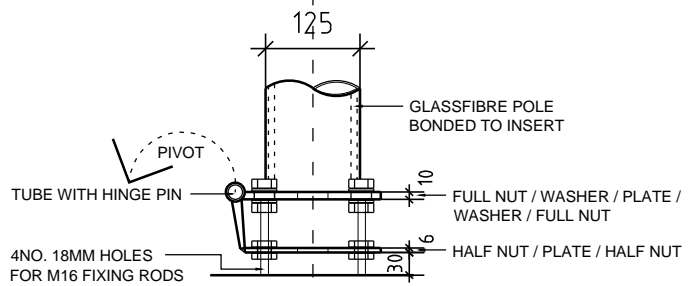
BASE PLATE / FOOT ELEVATION
