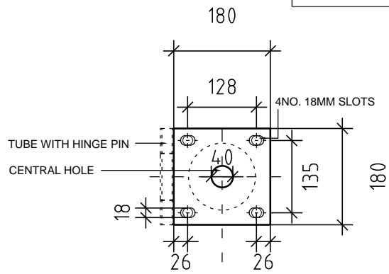
BASE PLATE PLAN
